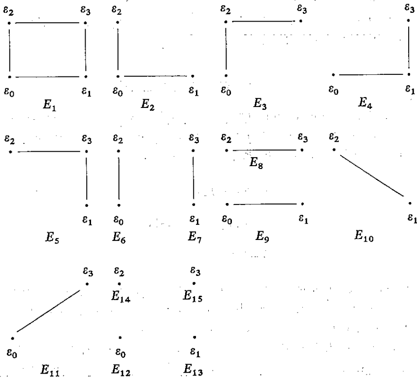
Fig. 5.1. Graphic representation of U(2)^9
