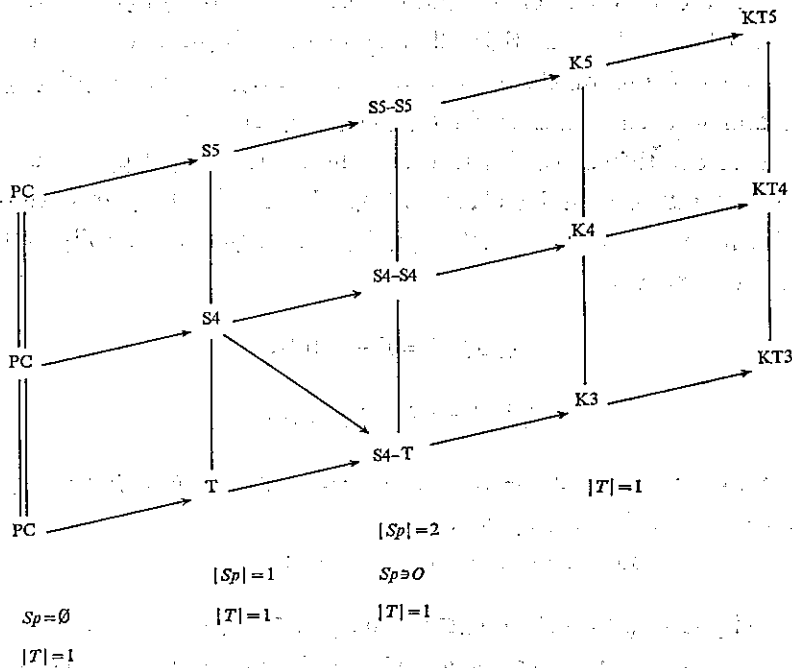
Fig. 1.1. Relation of KT_i to other modal logics
